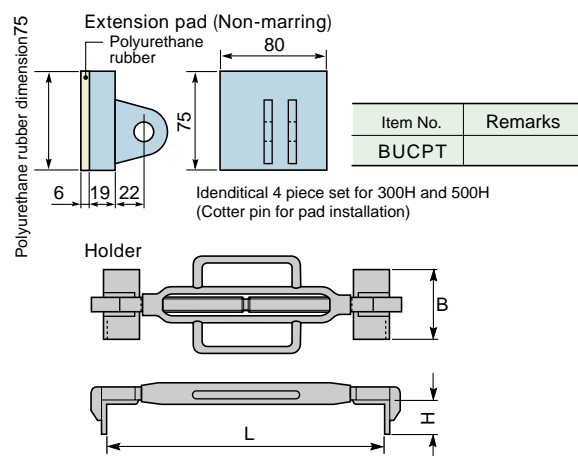
DIMENSIONS TABLE (Holder)
